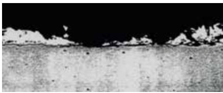
Microscopic picture view of galvanized steel after weathering
